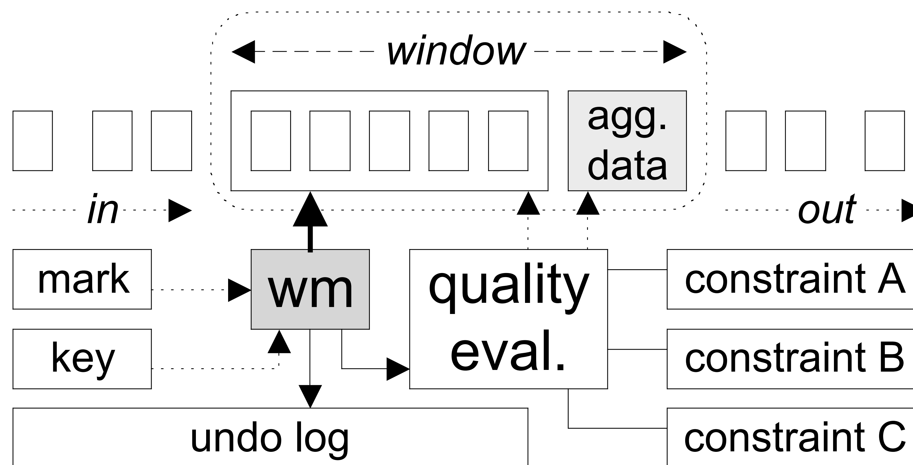
Sensor Stream Watermarking: Implementation
