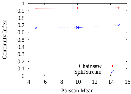
Fig. 7. Continuity Index using a configuration of an initial 80 nodes followed by other nodes joining based on a Poisson process
