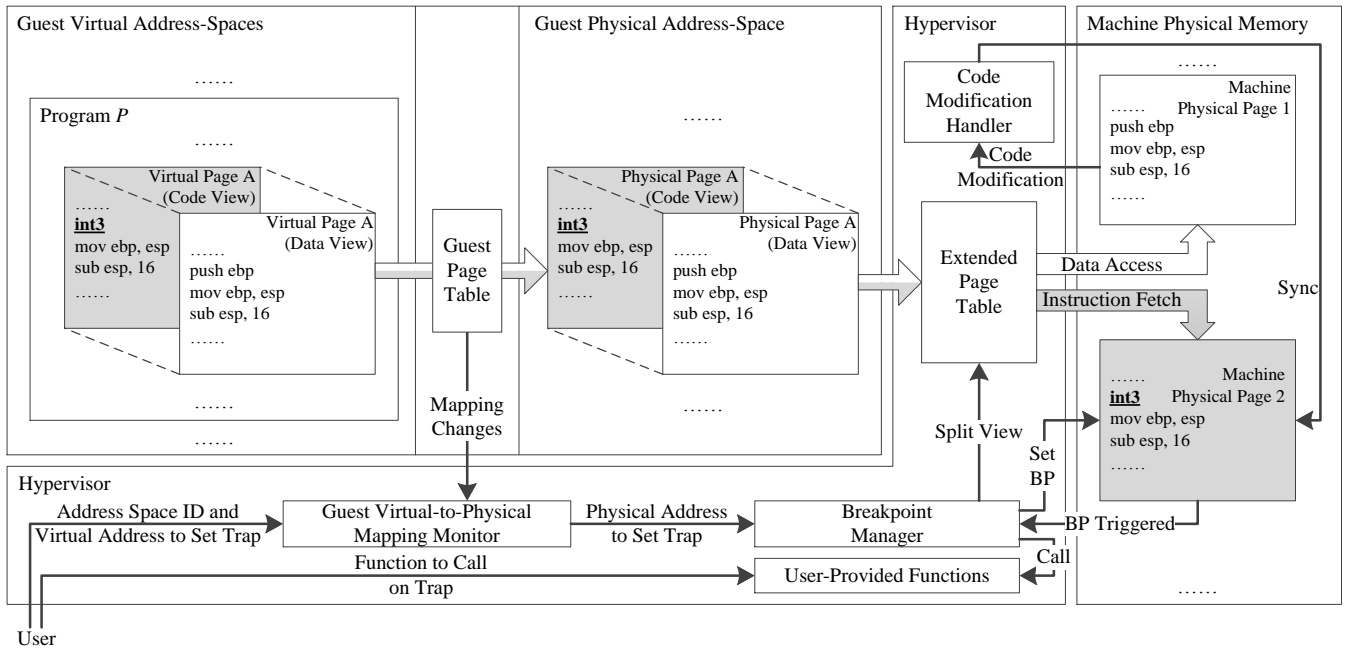
Figure 1: Overview of SPIDER.
