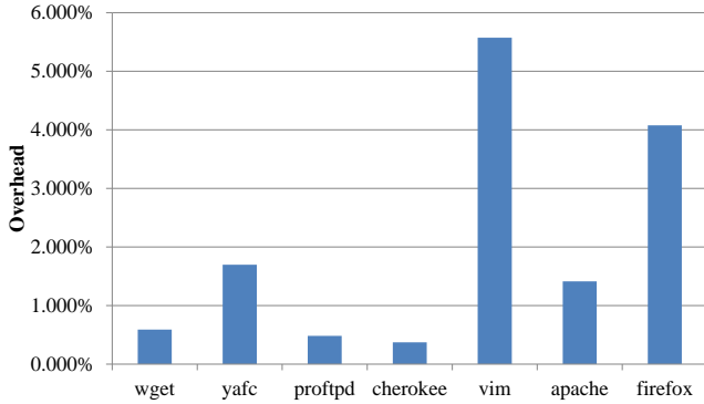
Figure 3: Overhead of using SPIDER to perform instrumentation for BEEP.
