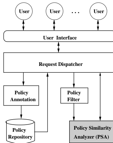
Fig. 1. EXAM Architecture
