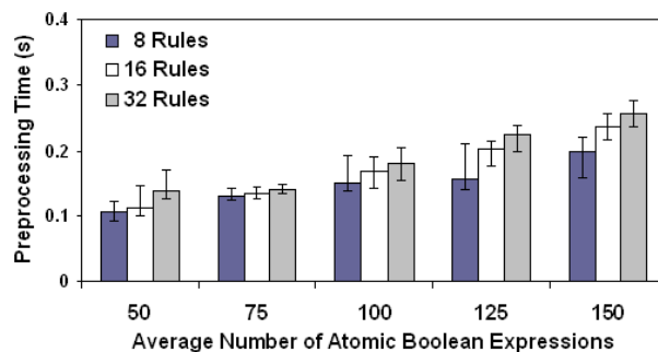
Fig. 10. Response Time Taken for Preprocessing a Pair of Policies
