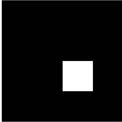
Figure 17. VW2D: T = 0
