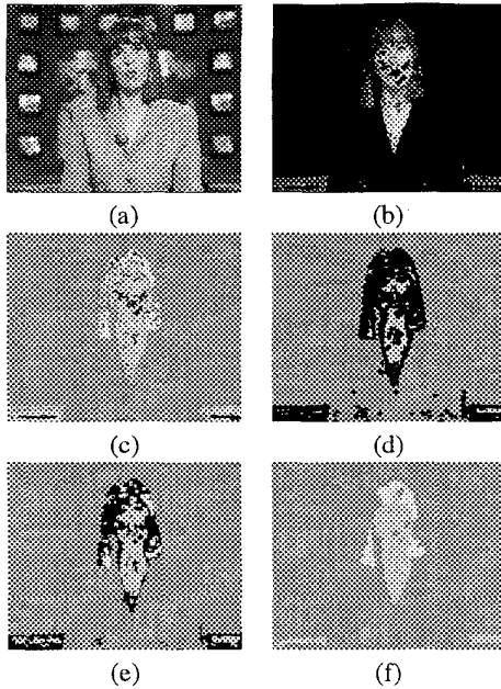
Fig. 6. (a) Original image. (b) Pixels detected as skin. (c) Segmentation after histogram clustering. (d) Label erosion of size 2 of c. (e) Label dilation of size 2 of d. (f) Watershed segmentation using the markers of e.
